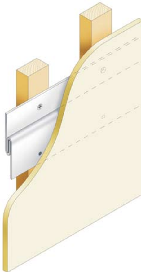
GA WP1 8.7mm wall to panel fixing distance
