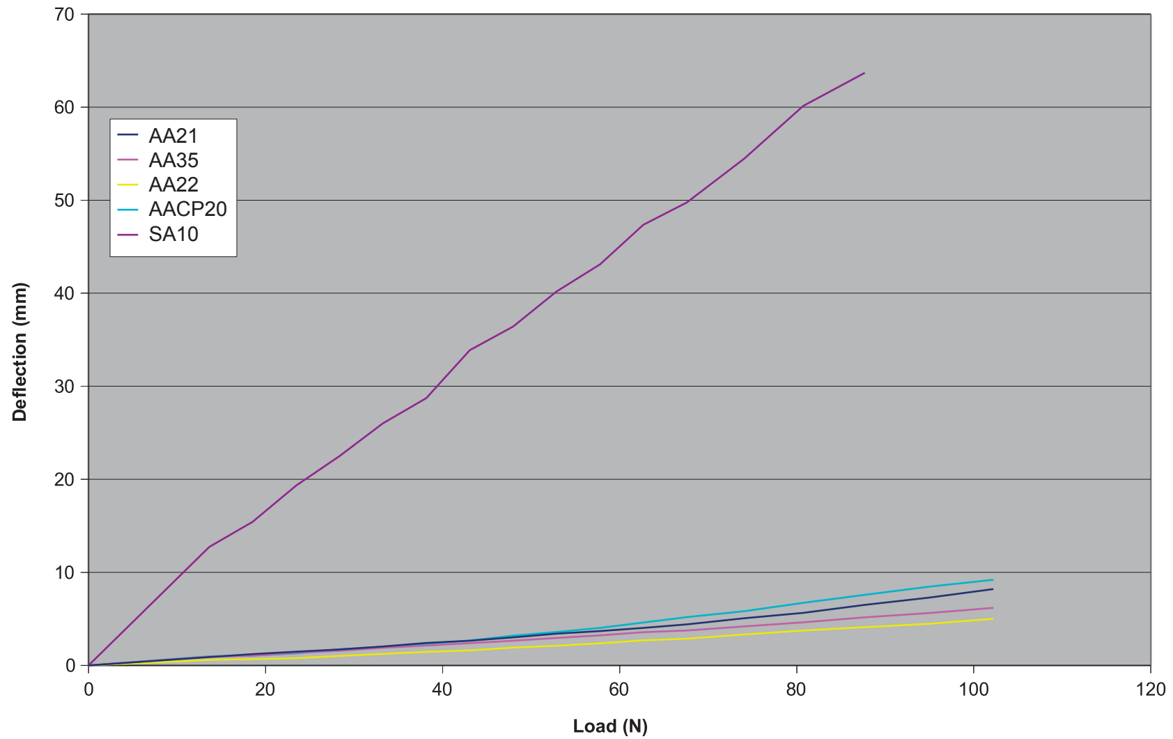
Graph 1 - Independent Test Results Aluminium Panels - Resistance to Deflection
