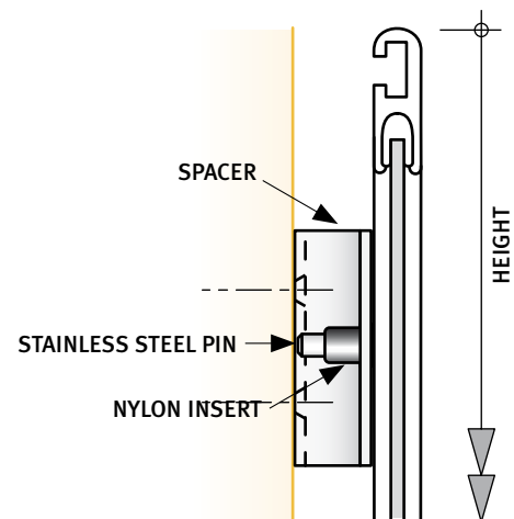
TYPICAL VERTICAL SECTION
